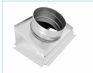
SLANT TOP OUTLET BOX
